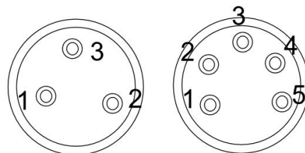
DMX input & XLR connector
