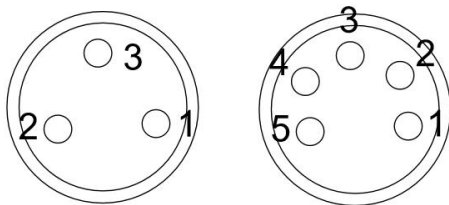
DMX output & XLR connector
