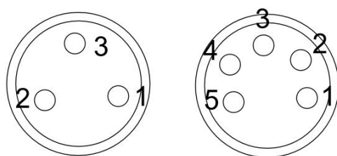
DMX output & XLR connector
